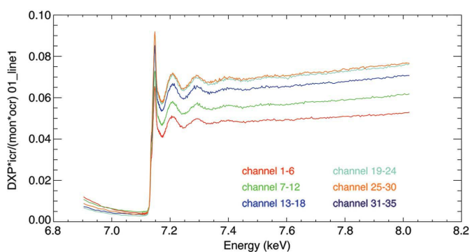
Figure 9 Spectra obtained from a single horizontal line of detector channels.
